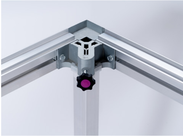
Corner section incl. leg mount without base board
